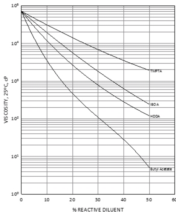
EBECRYL® 225 - VISCOSITY REDUCTION WITH REACTIVE DILUENTS
