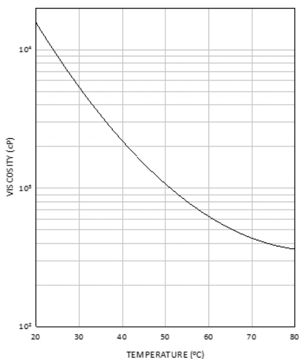
EBECRYL® 8315 - VISCOSITY VS. TEMPERATURE
