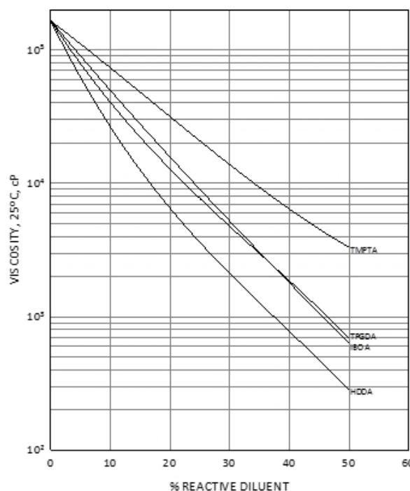
EBECRYL® 270 - VISCOSITY REDUCTION WITH REACTIVE DILUENTS
