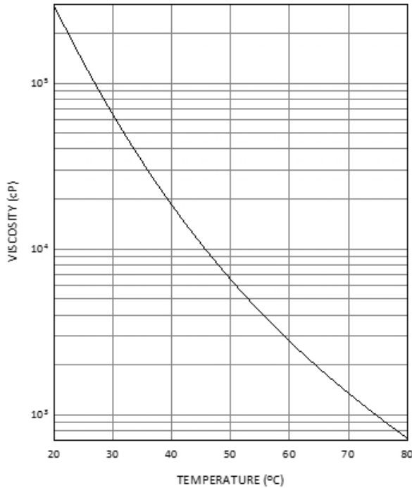
EBECRYL® 270 - VISCOSITY VS. TEMPERATURE
