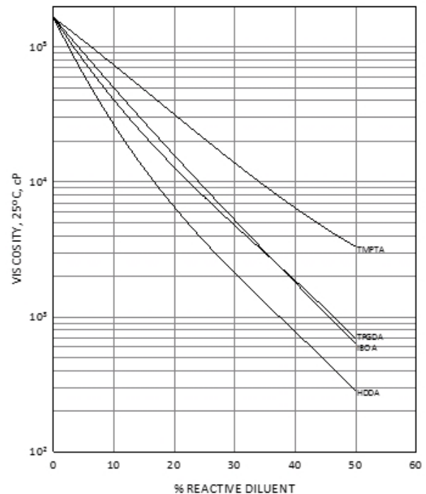
EBECRYL® 270 - VISCOSITY REDUCTION WITH REACTIVE DILUENTS
