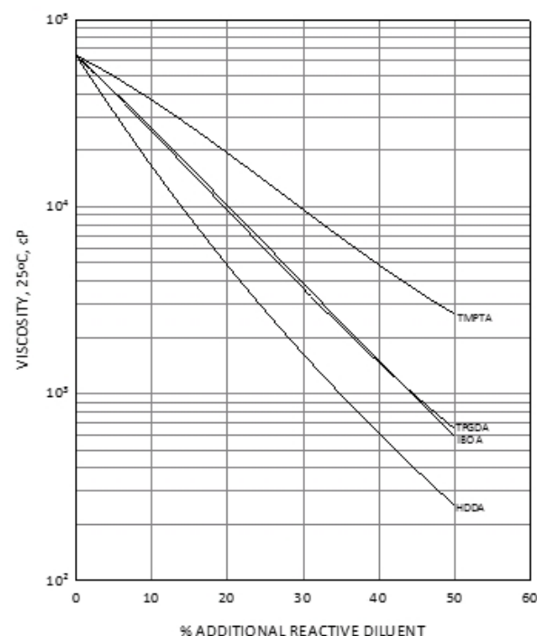
EBECRYL® 284 - VISCOSITY REDUCTION WITH REACTIVE DILUENT
