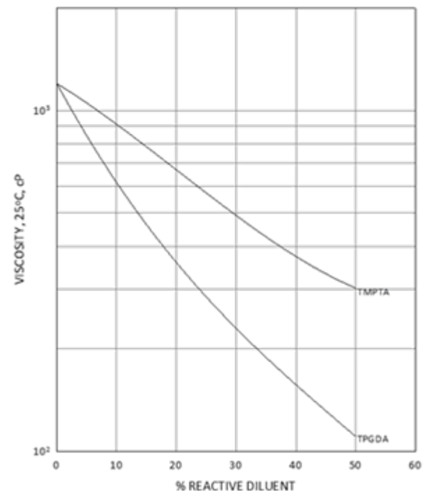
EBECRYL® 7100 - VISCOSITY REDUCTION WITH REACTIVE DILUENTS
