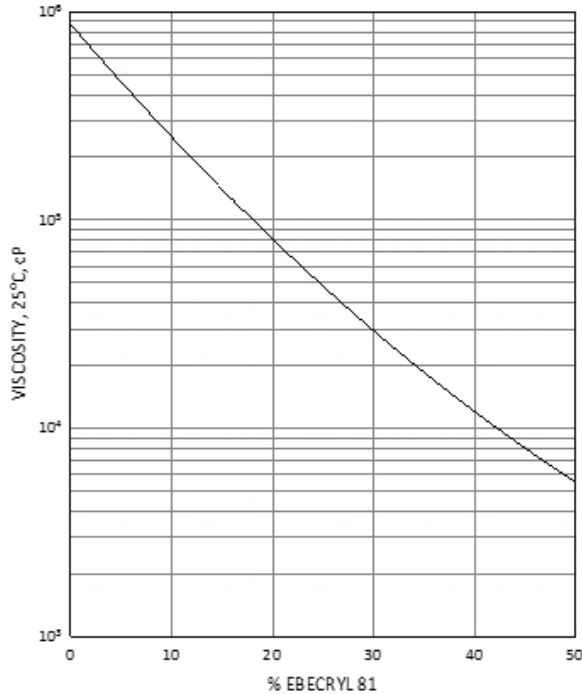
EBECRYL® 81 - VISCOSITY REDUCTION OF EBECRYL 3700
