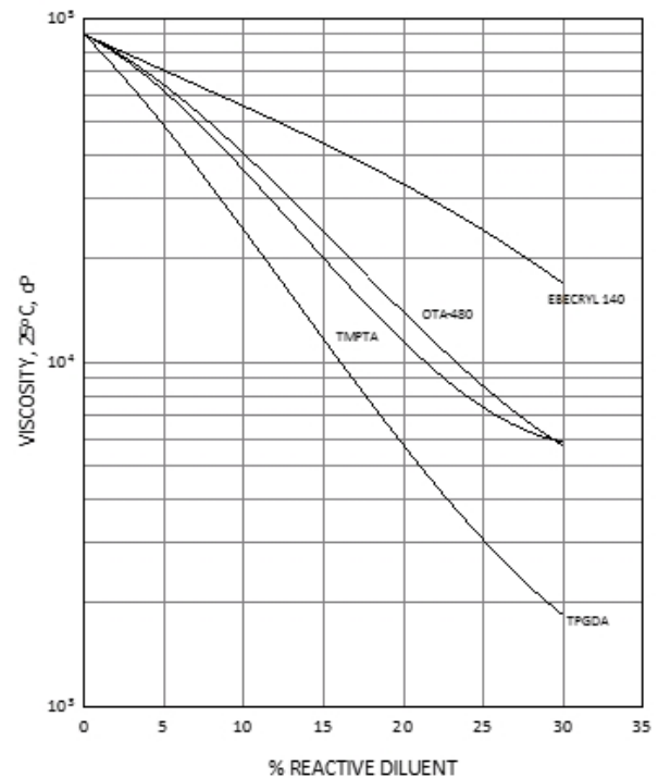
EBECRYL® 811 - VISCOSITY REDUCTION WITH REACTIVE DILUENTS
