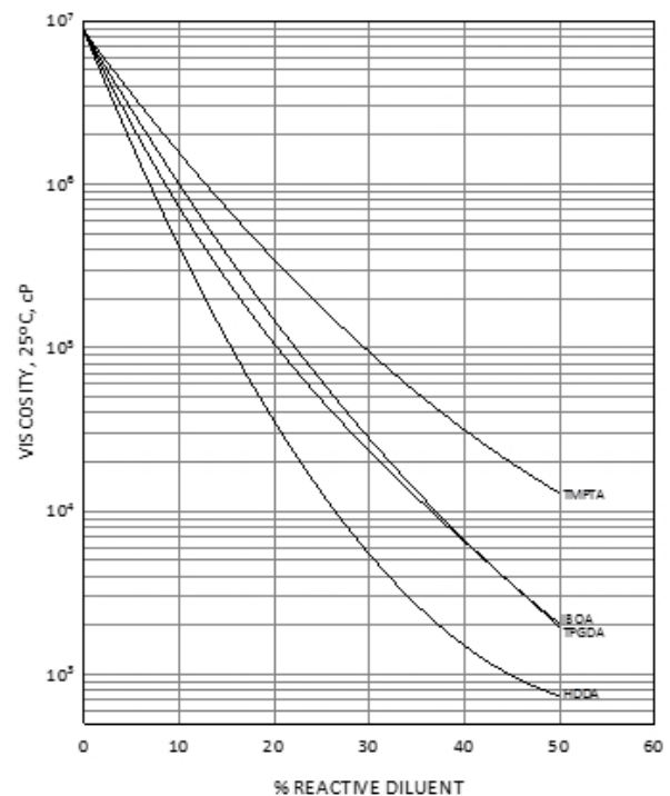
EBECRYL® 246 VISCOSITY REDUCTION WITH REACTIVE DILUENTS
