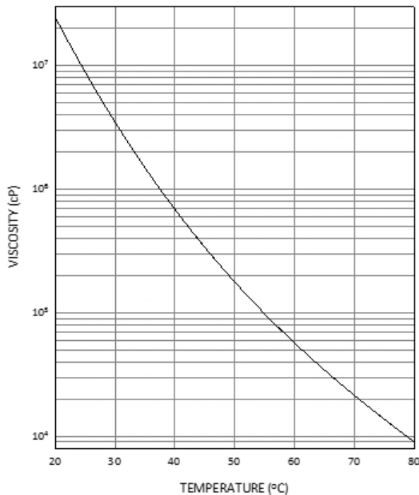
EBECRYL® 246 - VISCOSITY VS. TEMPERATURE
