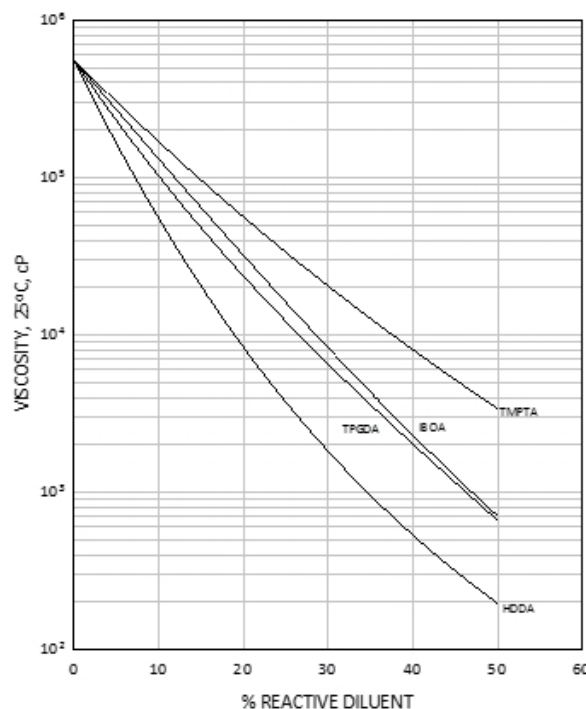
EBECRYL® 600 - VISCOSITY REDUCTION WITH REACTIVE DILUENTS
