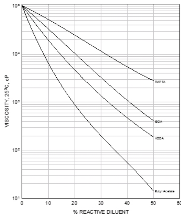
EBECRYL® 8602 - VISCOSITY REDUCTION WITH DILUENTS
