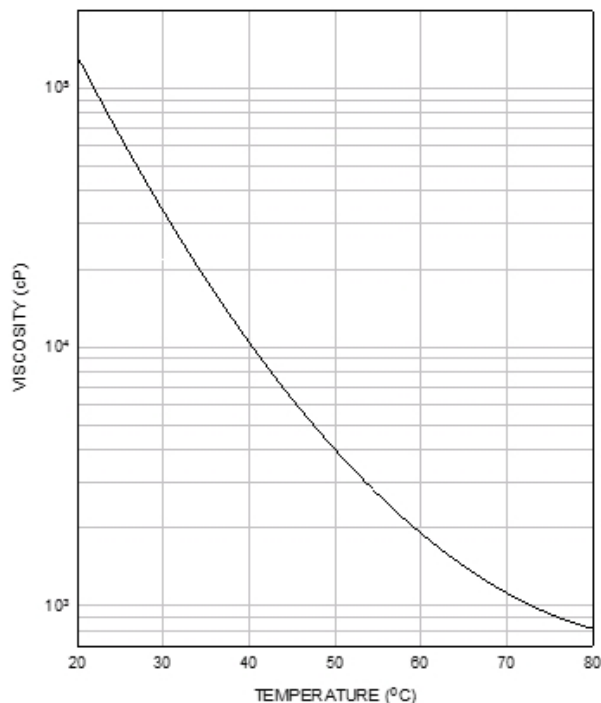
EBECRYL® 8602 - VISCOSITY VS. TEMPERATURE
